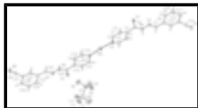
Fig. 1. A view of the Ag I coordination environment in the monomeric structure of (I), showing the atom-labelling scheme. Displacement ellipsoids are drawn at the 30% probability level.
